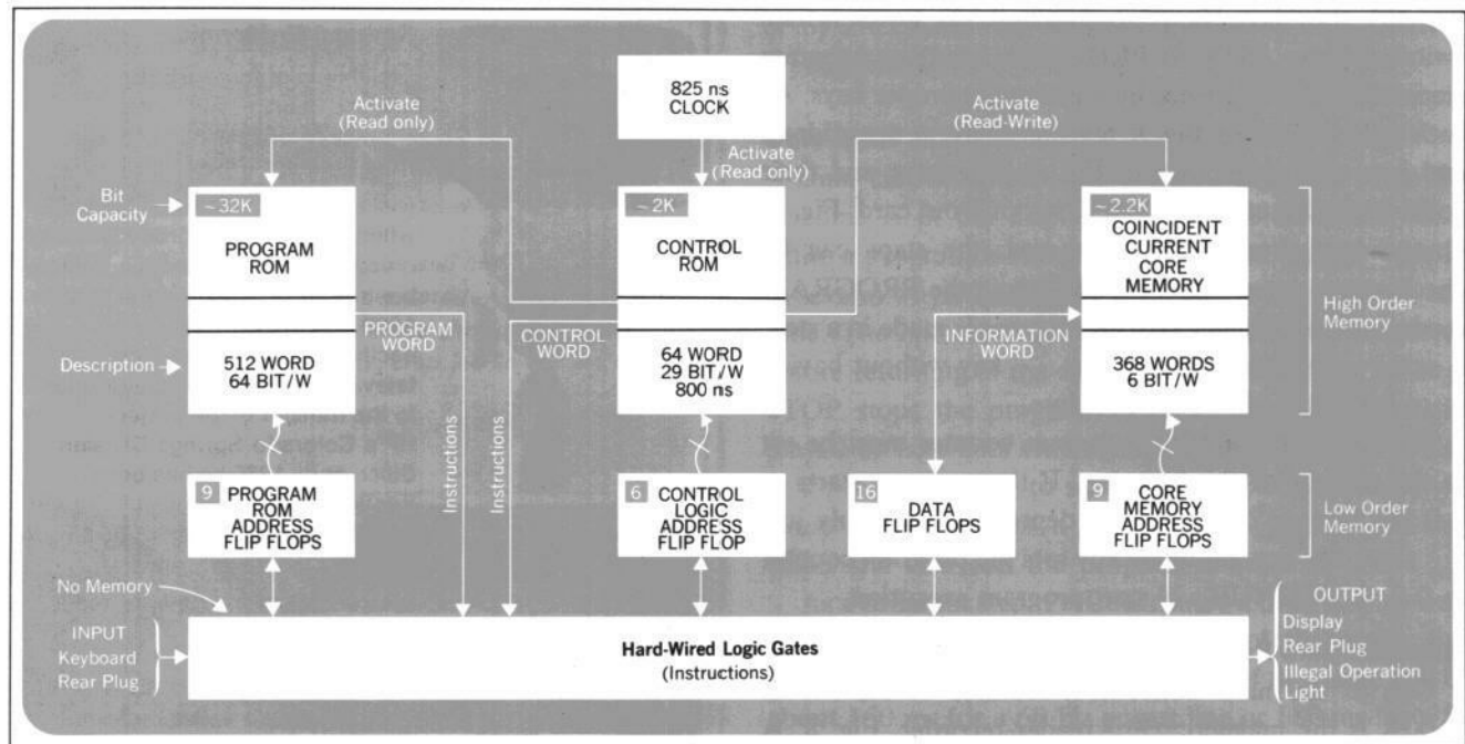
Fig. 1. Arithmetic processing unit block diagram. This system is a marriage of conventional, reliable diode-resistor logic to a 32,000-bit read-only memory and a coincident current core memory.
