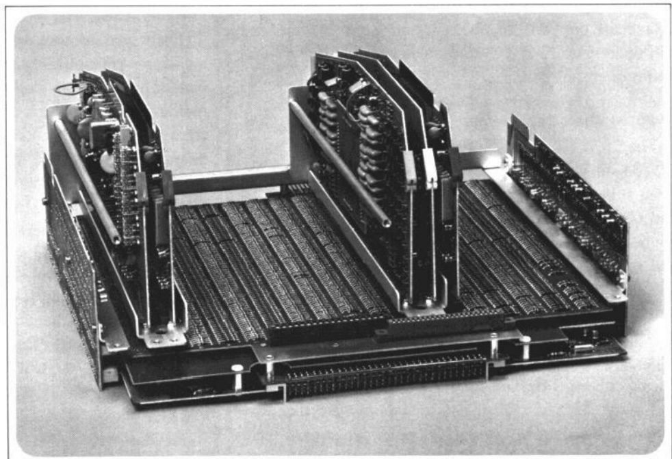
Fig. 2. Arithmetic unit assembly removed from the calculator.
