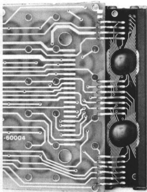
Fig. 1. HP-41C display assembly.
