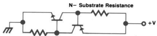
(b) Equivalent circuit of PNP parasitic device
