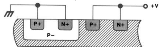
(a) CMOS cross-section
