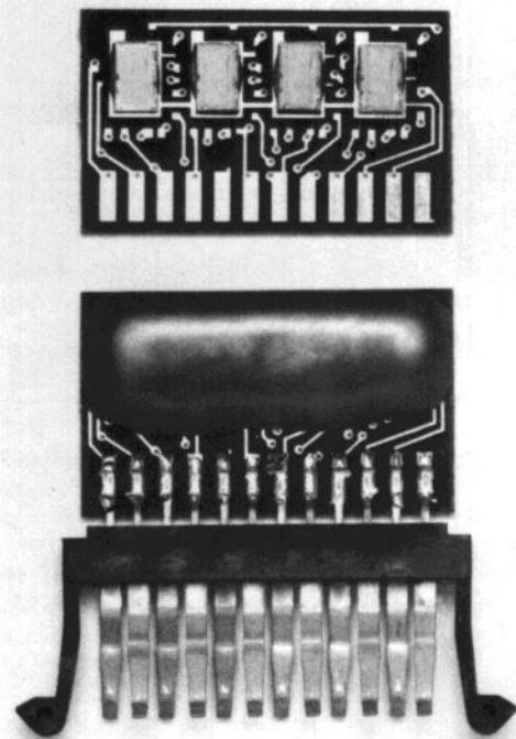
Fig. 2. RAM module contains four chips, each measuring 2.72 by 4.29 mm. Each chip contains sixteen 56-bit registers. There are 12-14 bonds per chip and ten connections via a reflow-soldered contact frame to the HP-41C. The substrate measures 23.37 x 13.72 x 0.79 mm.
