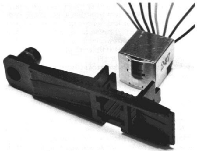
Fig. 4. Base assembly for card reader.
