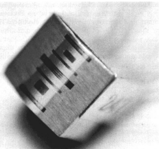
Fig. 3. A common read-after-write head design locates the read and write gaps on opposite sides of the head's crown. The head used in the HP-75 has these gaps located on the crown as shown.
